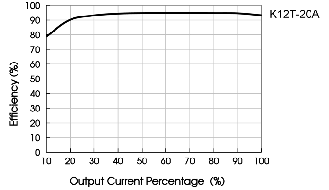
Efficiency Vs Output Load ( V_{in}=12V, V_{out}=3.3V )
