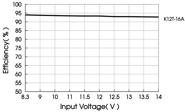
Efficiency Vs input Voltage ( V_{out}=3.3V, I_o=16A )
