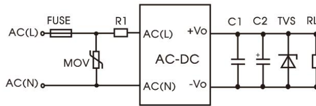
Fig. 2: EMC application circuit with higher requirements
