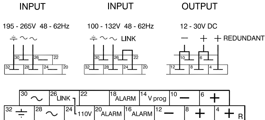
H 15 connector
